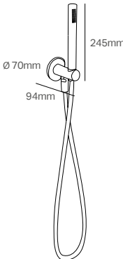
Doccino Hand shower
